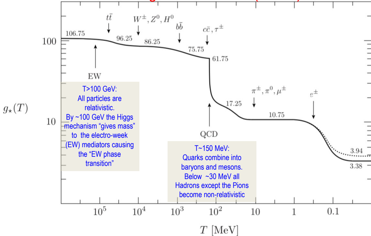
Figure 3.4: Evolution of relativistic degrees of freedom g_*(T) assuming the Standard Model particle content. The dotted line stands for the number of effective degrees of freedom in entropy a_{\text{eff}}(T) .
