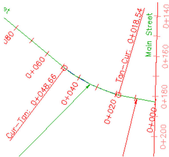
Geometry point labels with abbreviations modified in drawing settings
