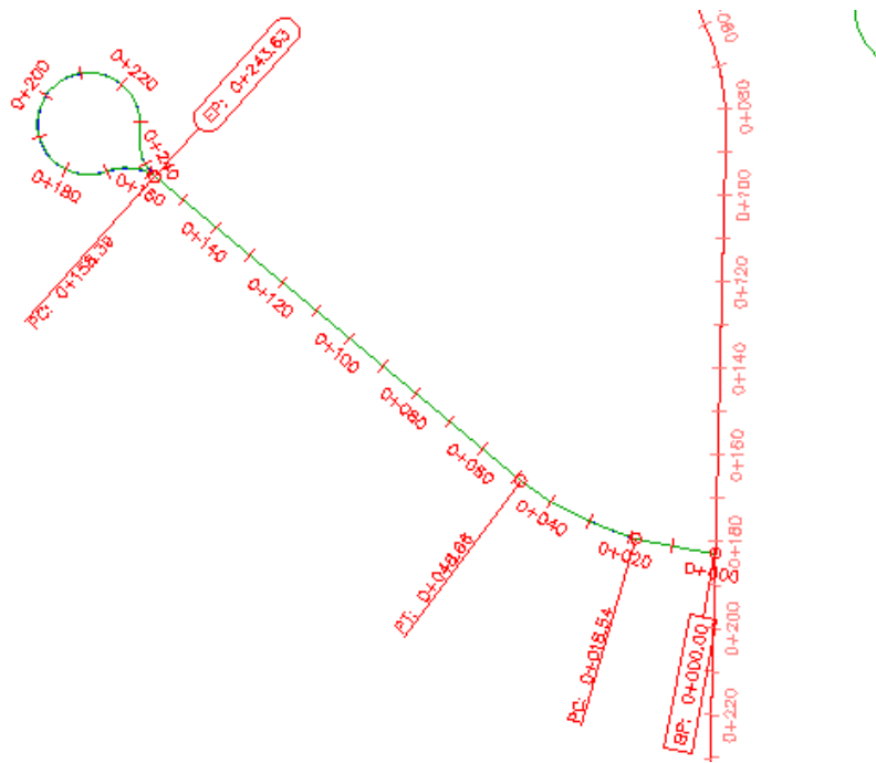
Alignment with modified label set
