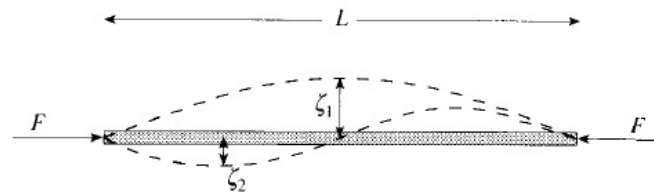
Figure 8.2 A strut under compression. The broken curves suggest two normal modes of flexural distortion, corresponding to n = 1 and n = 2 .
