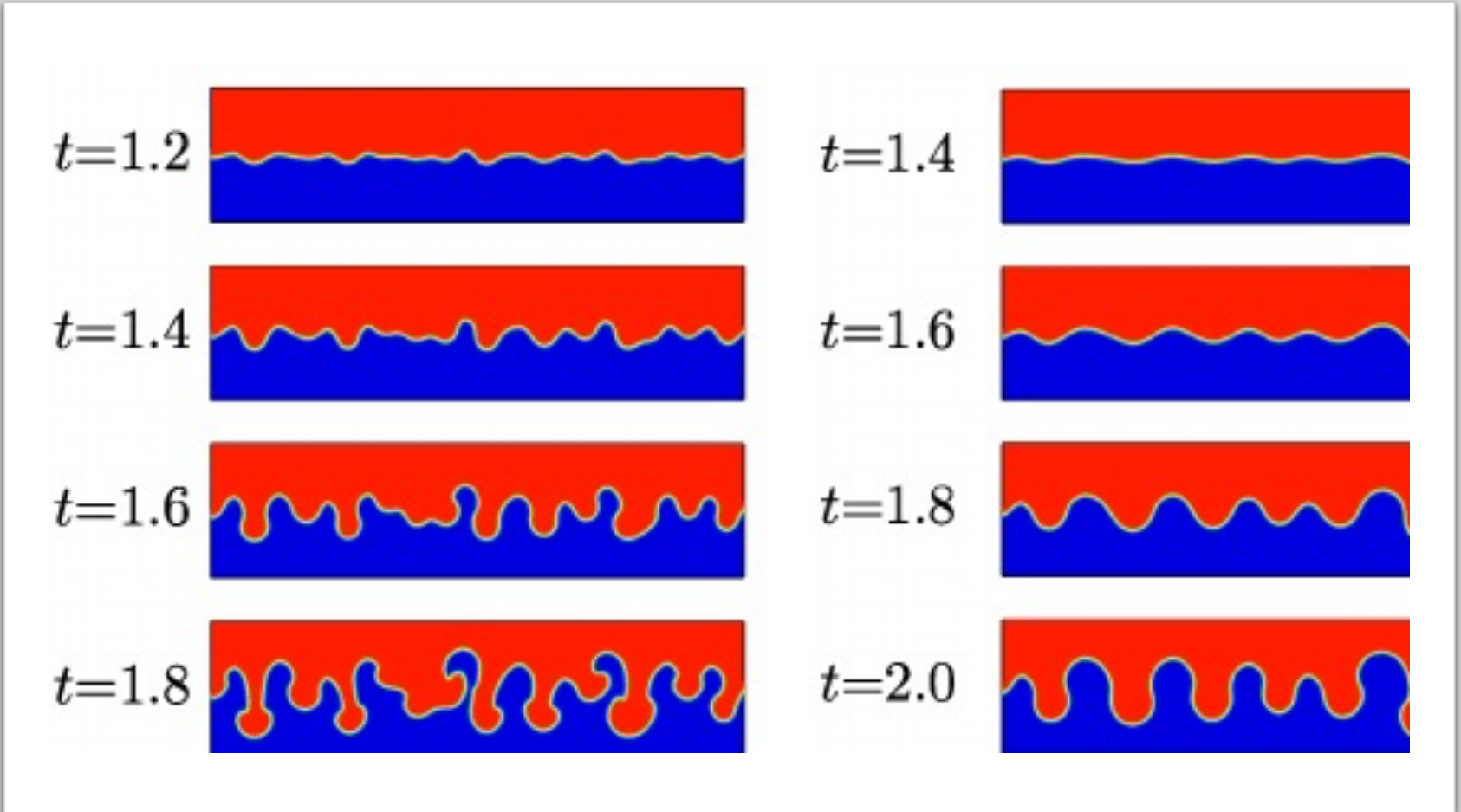
Rayleigh-Taylor
