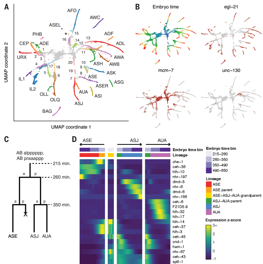
Fig. 3. Developmental trajectories of ciliated neurons.
