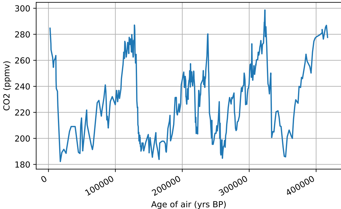
Evolution of the concentration of CO2 in Vostok
