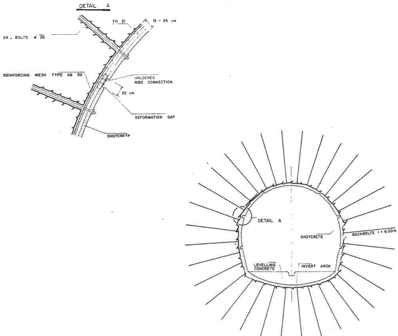
Fig. 8. Where large deformations occur in the tunnel walls it is important to have a flexible lining. The figure is an example from the Taurn tunnel where the initial lining (by shotcrete and rock bolts) has been designed with a longitudinal joint. (after Amberg and Cristini, 1986)
