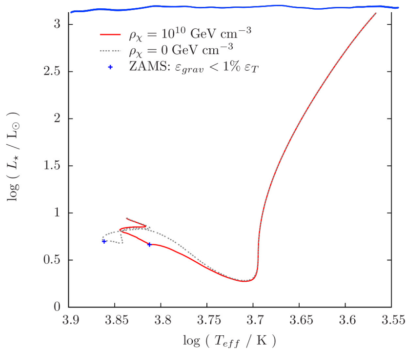
Figure 4. Hertzsprung-Russell diagram of the formation and evolution through the main-sequence of a star of 1.5M_{\odot} . The red line represents the path taken by the star when it is embedded in a DM halo of \rho_{\chi} = 10^{10} \text{ GeV cm}^{-3} , the gray dashed line is the classical evolution, i.e, without the presence of dark matter particles and the blue symbols "+" represent the ZAMS position on each case. Credits: [1]
