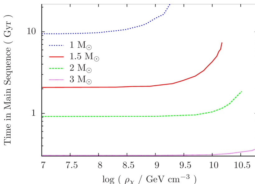
Figure 3. Time that stars of masses 1M_\odot , 1.5M_\odot , 2M_\odot and 3M_\odot spend in the main-sequence when embedded in dark matter halos of densities between 10^7 \text{ GeV cm}^{-3} and 10^{11} \text{ GeV cm}^{-3} . Credits: [1]
