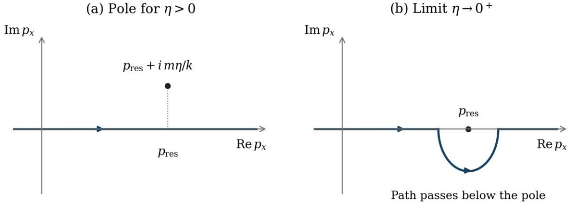
Figure 2.6.2. The resonant pole and the causal momentum contour in (2.6.53). The arrows indicate integration from left to right. In the limit the contour passes below the pole, giving the principal value and the negative imaginary term.
