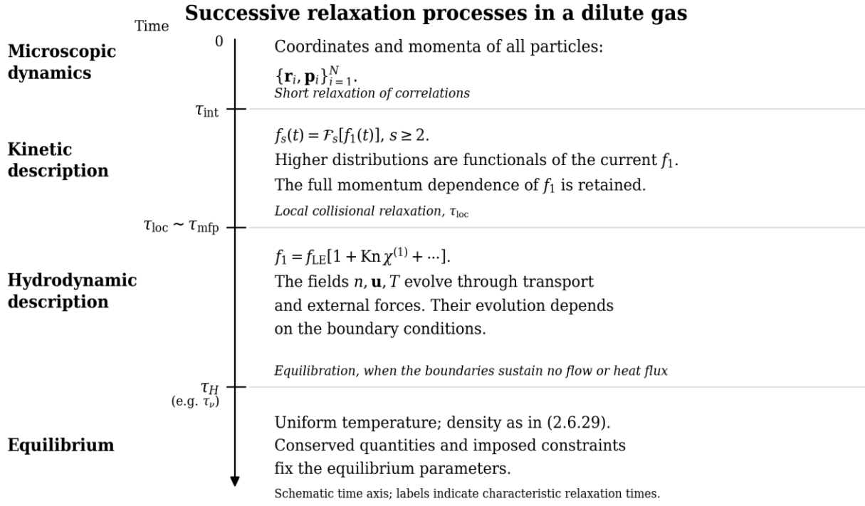
Figure 2.8.1. Successive descriptions and characteristic relaxation times. The dilute-gas estimates of §2.4 give \tau_{int} \sim 7 \times 10^{-13} s and \tau_{loc} \sim \tau_{mfp} \sim 1.4 \times 10^{-10} s. As an illustration of the much longer hydrodynamic relaxation, the shear disturbance (2.8.61), with wavelength 2 mm, has k = \pi/(1 \text{ mm}) . Taking v \simeq 1.4 \times 10^{-5} \text{ m}^2 \text{ s}^{-1} gives \tau_H = \tau_v = 1/(vk^2) \simeq 7 \times 10^{-3} s. The time axis is schematic. The marked times characterize relaxation processes; equilibrium is approached over several decay times.
