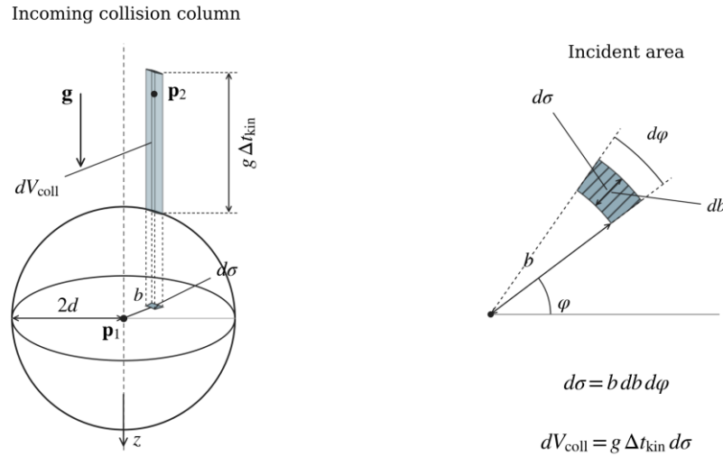
Figure 2.4.1. The shaded column contains the initial partner positions from which entry through the selected sphere patch occurs during \Delta t_{\text{kin}} . The right panel shows its transverse area d\sigma = b db d\varphi . The positive z direction is along g ; the labels p_1, p_2 identify the initial particle momenta.
