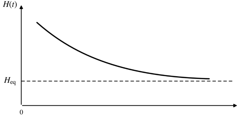
Figure 2.5.1. Schematic H(t) for relaxation to uniform Maxwell equilibrium. The dashed line marks H_{\text{eq}} ; the curve does not represent a specified relaxation law.
