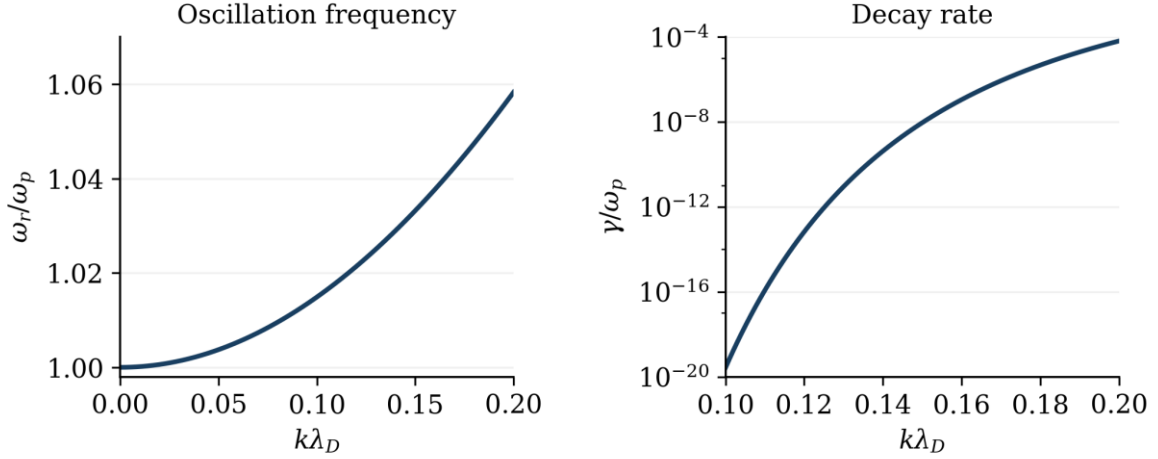
Figure 2.6.3. The long-wavelength estimates (2.6.58) and (2.6.64), plotted for k\lambda_D \leq 0.20 . The decay-rate panel uses a logarithmic vertical scale. Both curves are evaluated using the stated asymptotic formulas.
