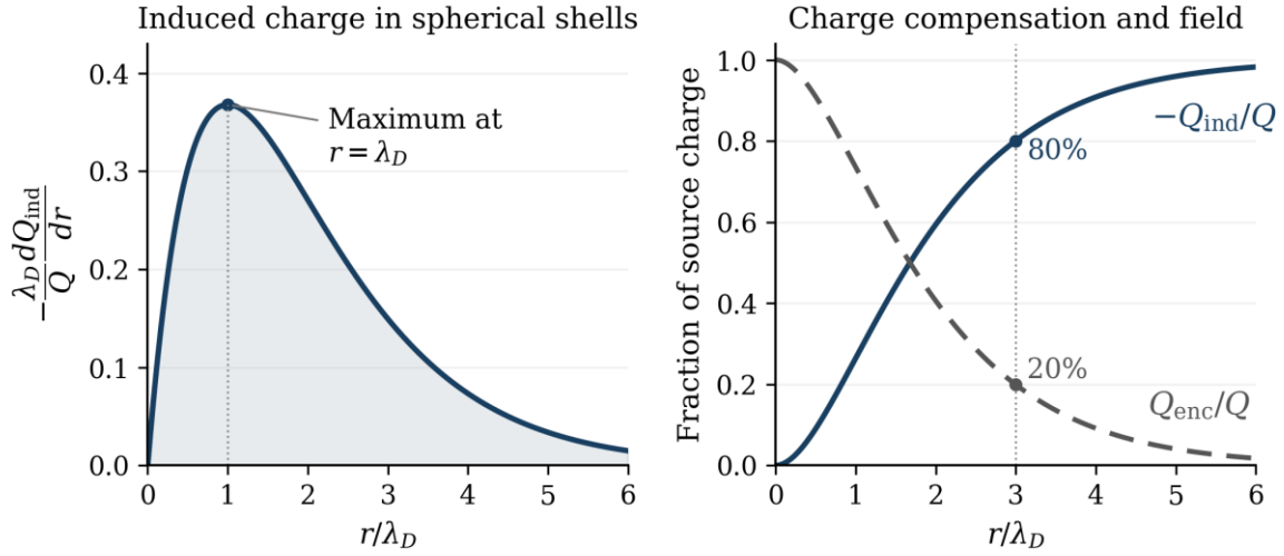
Figure 2.6.1. Screening as charge compensation in the linear point-source solution. Left: the normalized magnitude of the induced charge per radial interval, (2.6.32), is largest at one Debye length. Right: the accumulated compensating fraction -Q_{\text{ind}}/Q and the remaining charge fraction Q_{\text{enc}}/Q from (2.6.30) and (2.6.31). The latter is also the electric field relative to its vacuum value. At r = 3\lambda_D , about 80% of the source charge is compensated and about 20% of its vacuum field remains.
